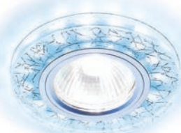
S226 W/CH/C D 90 mm H 22 mm A 65 mm 3W LED COLD + LED MR16 G5.3/GU10
